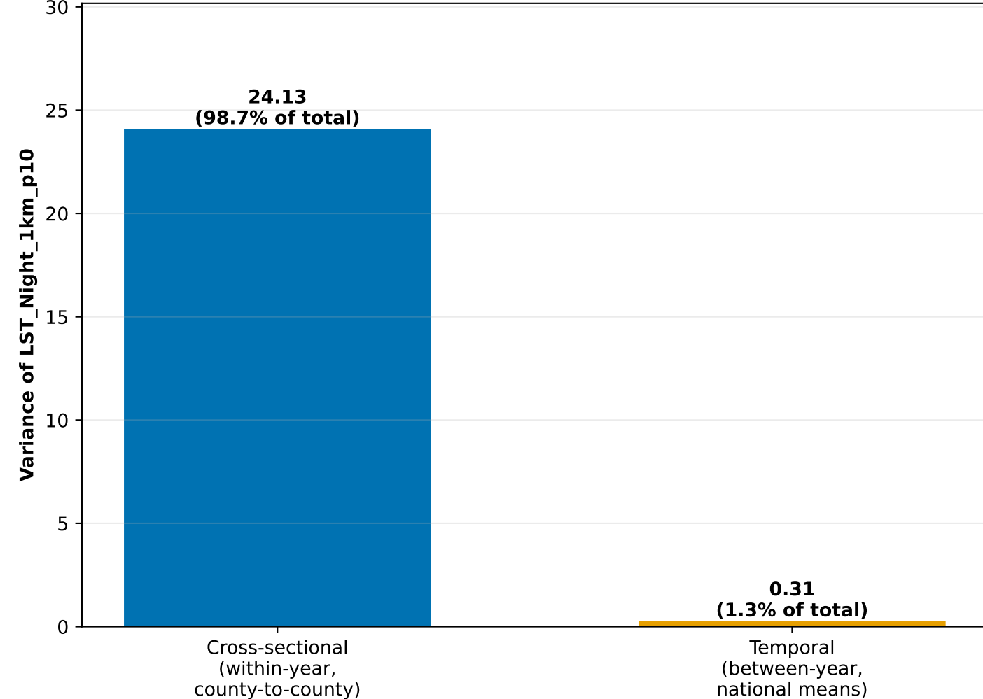
(B) The predictive signal is spatial, not temporal
