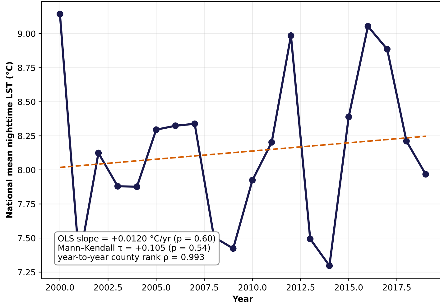
(A) No material national LST trend over 20 years
