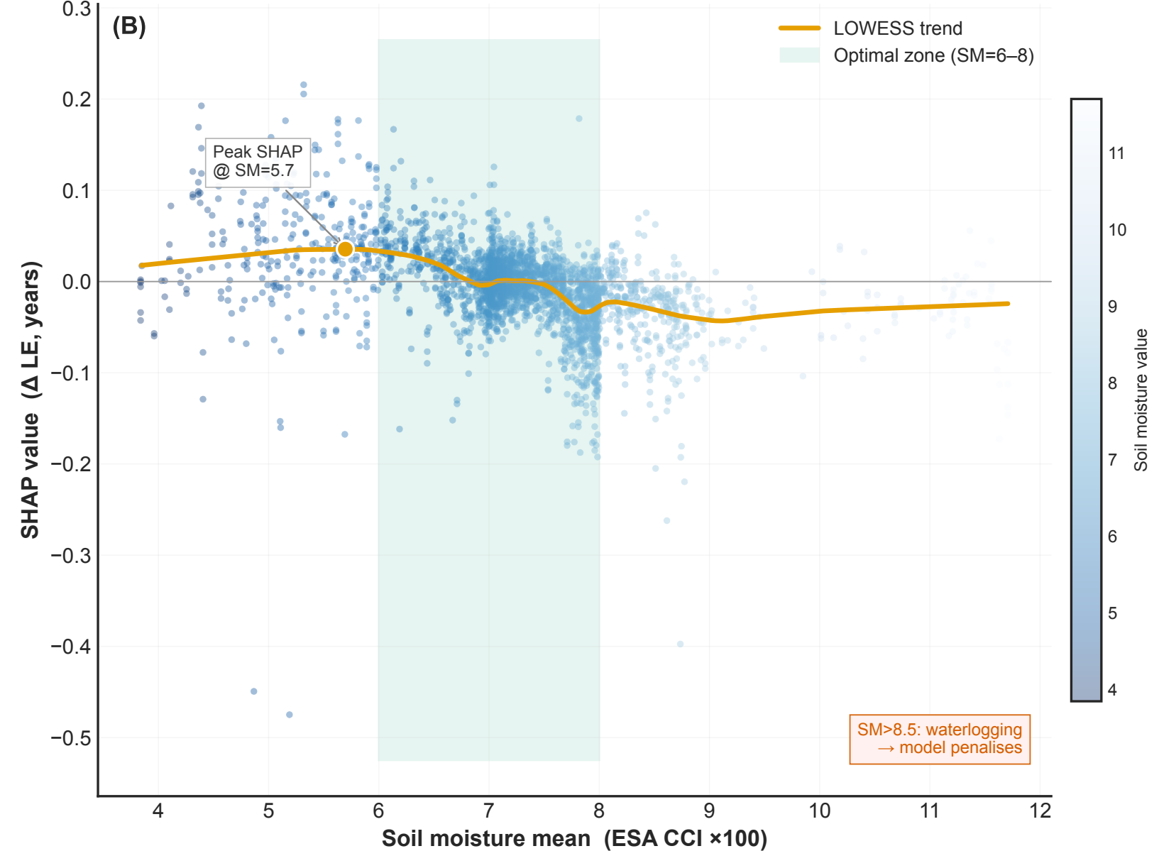
Model-attributed soil effect: inverted-U shape
