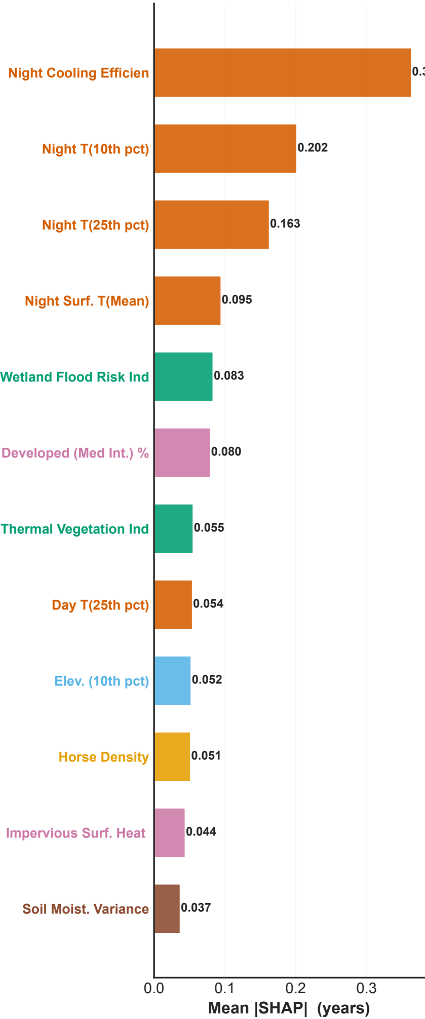
(D2) Individual mean |SHAP|
