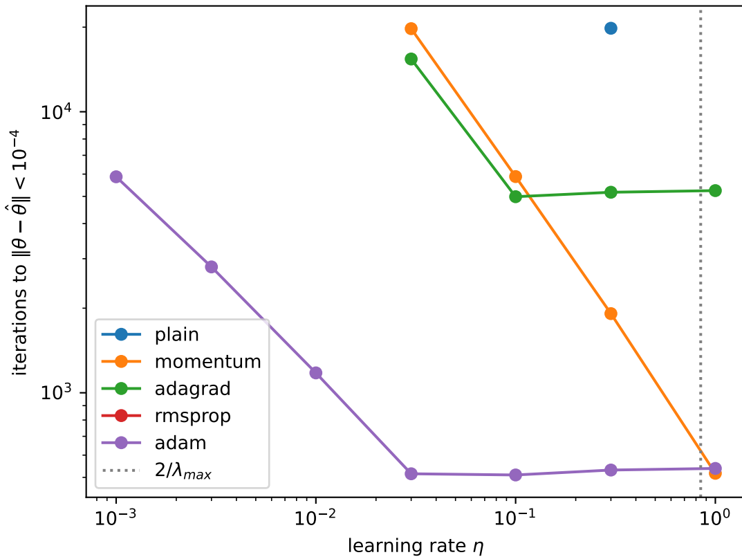
OLS, degree 5
