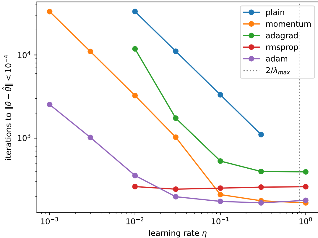
Ridge, degree 5
