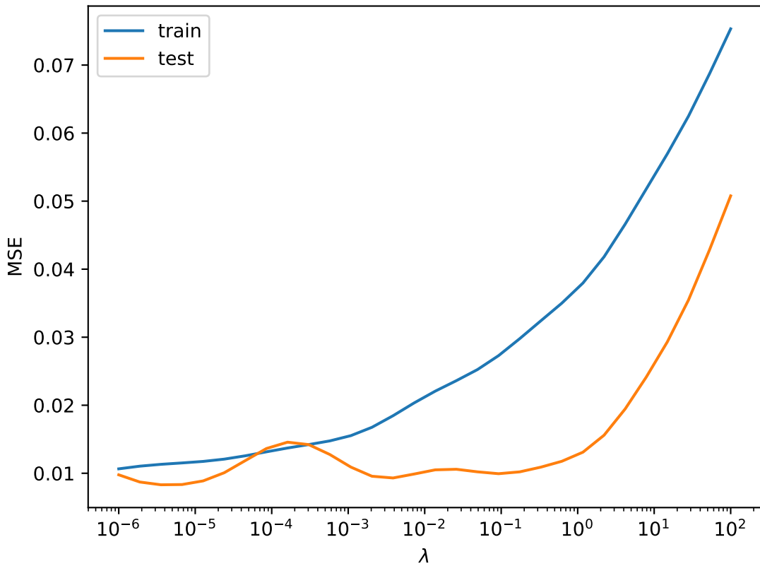
Ridge, degree 15
