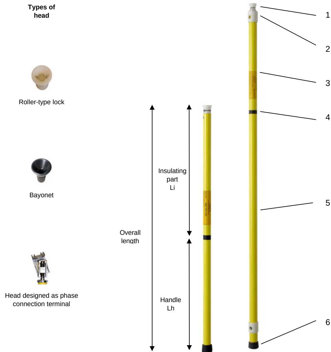
Fig. 1: Earthing stick
