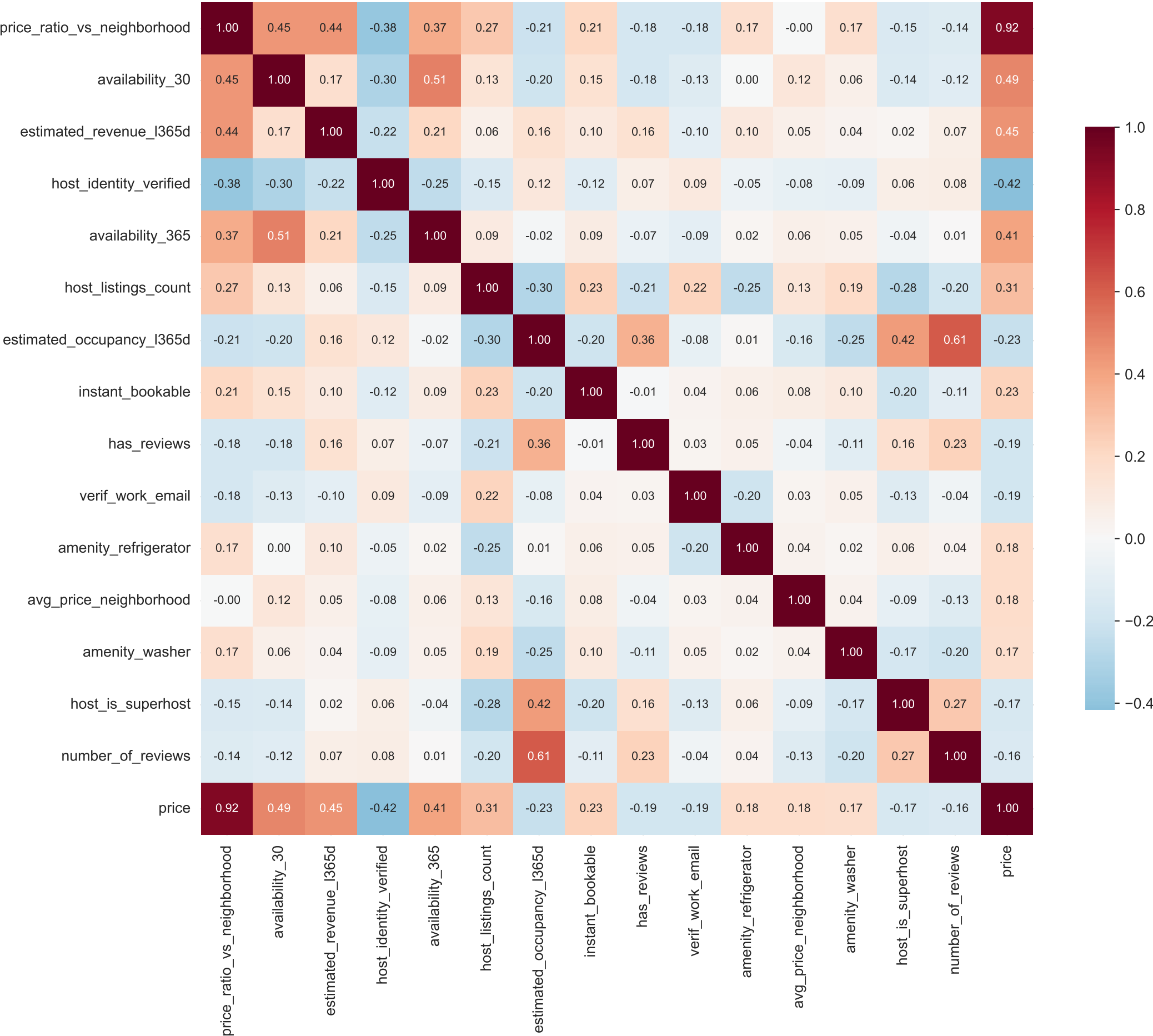
Matriu de correlacions (top 15 variables + price)
