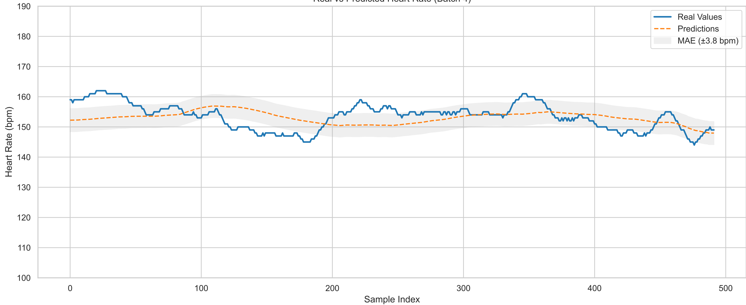
Real vs Predicted Heart Rate (Batch 4)
