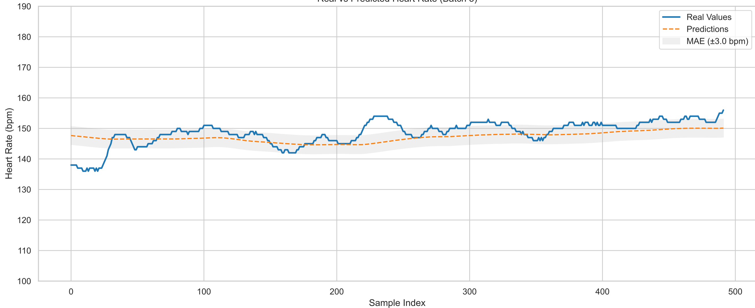
Real vs Predicted Heart Rate (Batch 3)
