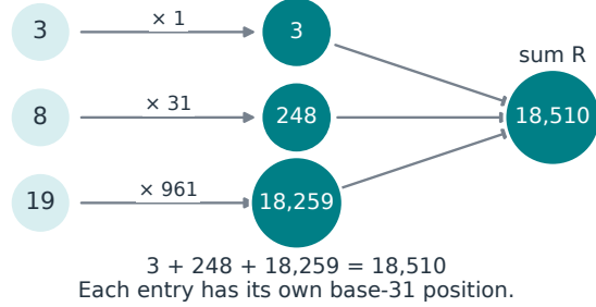
B. Second query: assign distinct digit weights
