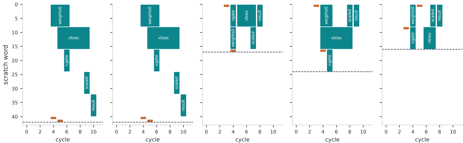
Top: engine x cycle, operation identifiers in each issue slot. Bottom: each value occupies its words from its write cycle to its last read (teal: 8-word vectors; orange: scalars). Dashed line: footprint S.
