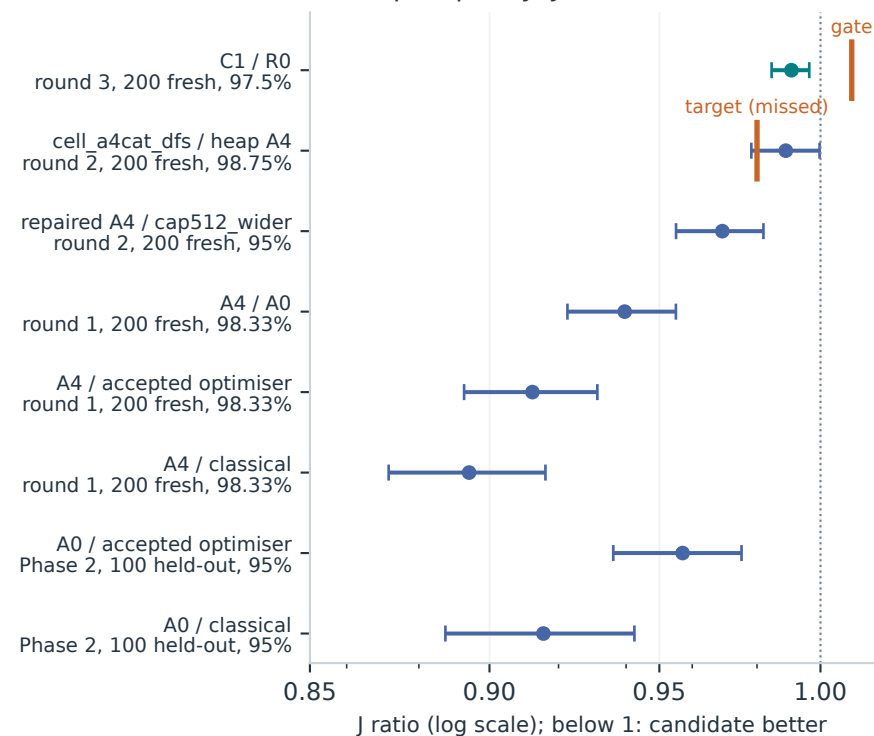
A. Output quality: J ratio, candidate / control
