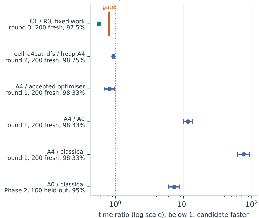
B. Compile time: candidate / control
