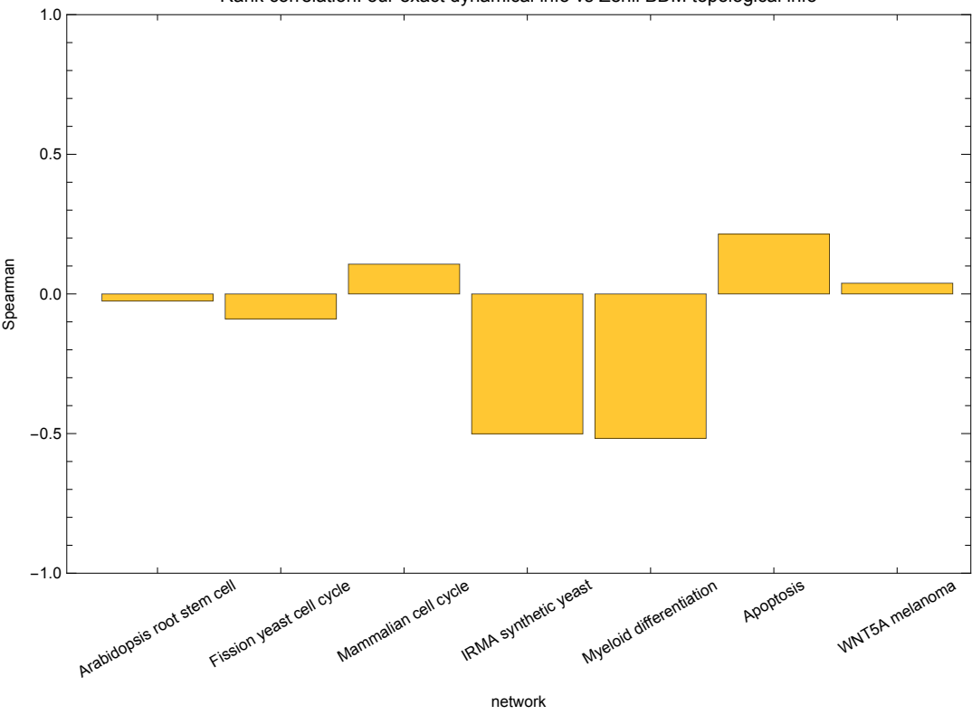
Rank correlation: our exact dynamical info vs Zenil BDM topological info
