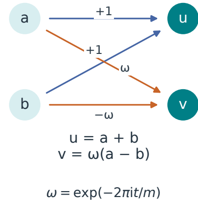
B. Read one butterfly
