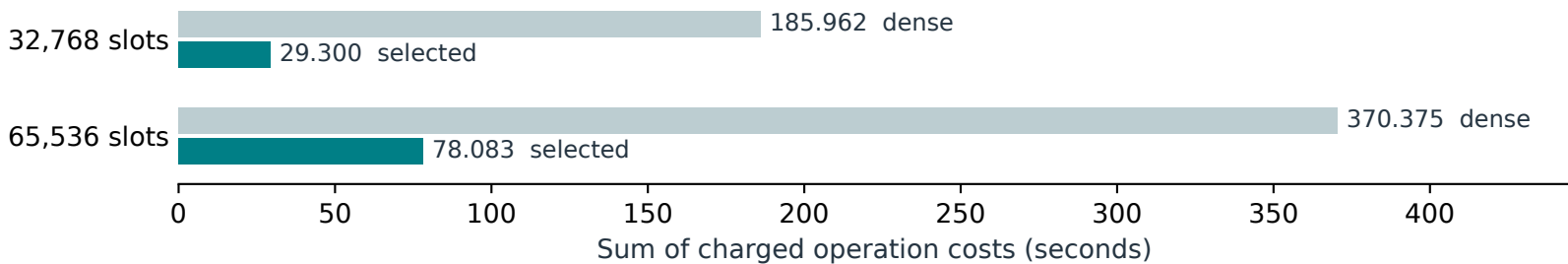
D. Estimated serial work under the same operation costs
