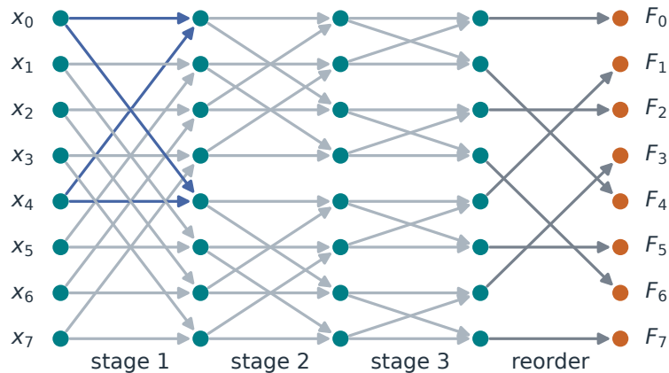
A. An eight-slot Fourier network
