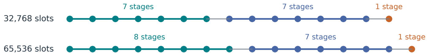
C. At the target sizes, fuse adjacent stages into three linear maps
