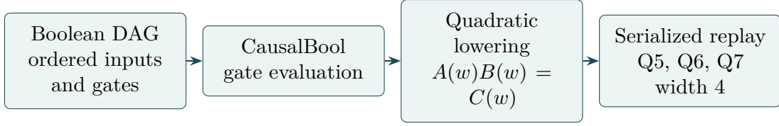
Figure 5: CausalBool-assisted arithmetic route. The Boolean DAG is evaluated through the existing CausalBool gate semantics and lowered to the frozen quadratic-row representation. Independent serialized replay verifies Q5 and Q6 at their stated widths and Q7 exhaustively at width four.
