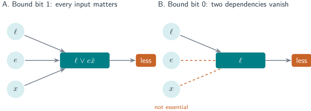
Figure 5: The comparator specialises itself. Both panels show the outgoing “less” of one comparison step, whose inputs are the incoming “less” \ell , the incoming “equal” e , and the value bit x . The cell is stated only as the meaning of a running comparison; the bound bit is a constant of the position, and nothing else is said. Against a bound bit of one the method finds all three inputs essential and names a two-clause form. Against a bound bit of zero it finds e and x inessential and returns \ell alone: below the bound one stays below, and no zero bound bit can create a new strict inequality. The orange dashed edges are the dependencies the method removed. They were not removed by an optimisation pass; the cofactor test simply did not find them.
