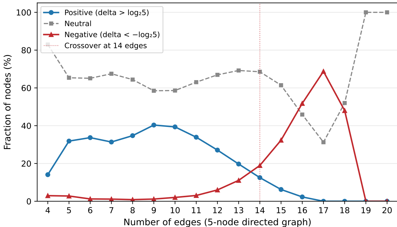
Figure 4D — BDM perturbation sign vs edge density (exhaustive 5-node directed graphs, n = 9364 , authors' deltas)
