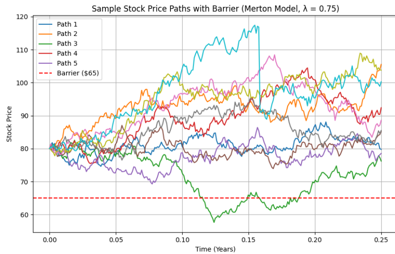
Figure 9: Sample Stock Price Paths with Barrier (Merton Model, \lambda = 0.75 )
