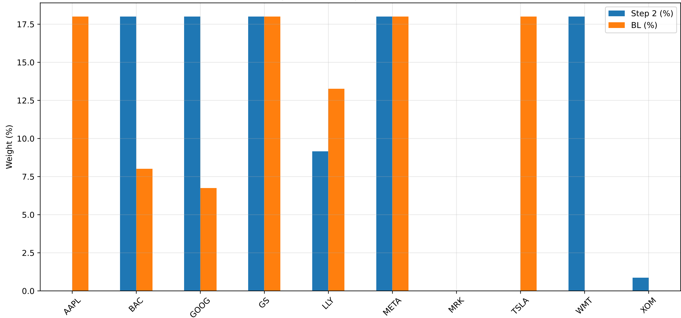
Portfolio Weights: Part 1 Step 2 vs Black-Litterman (Part 4)
