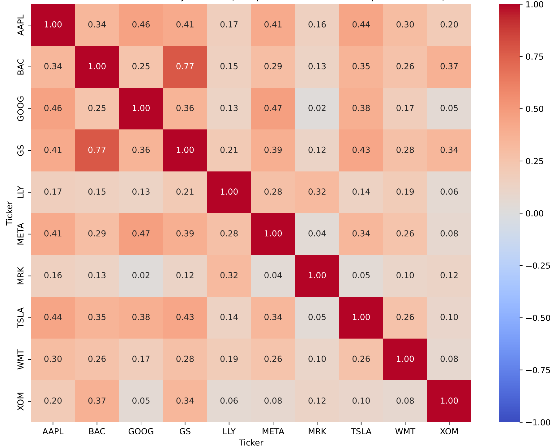
Correlation Matrix of Daily Returns (1 September 2023 to 30 September 2025)
