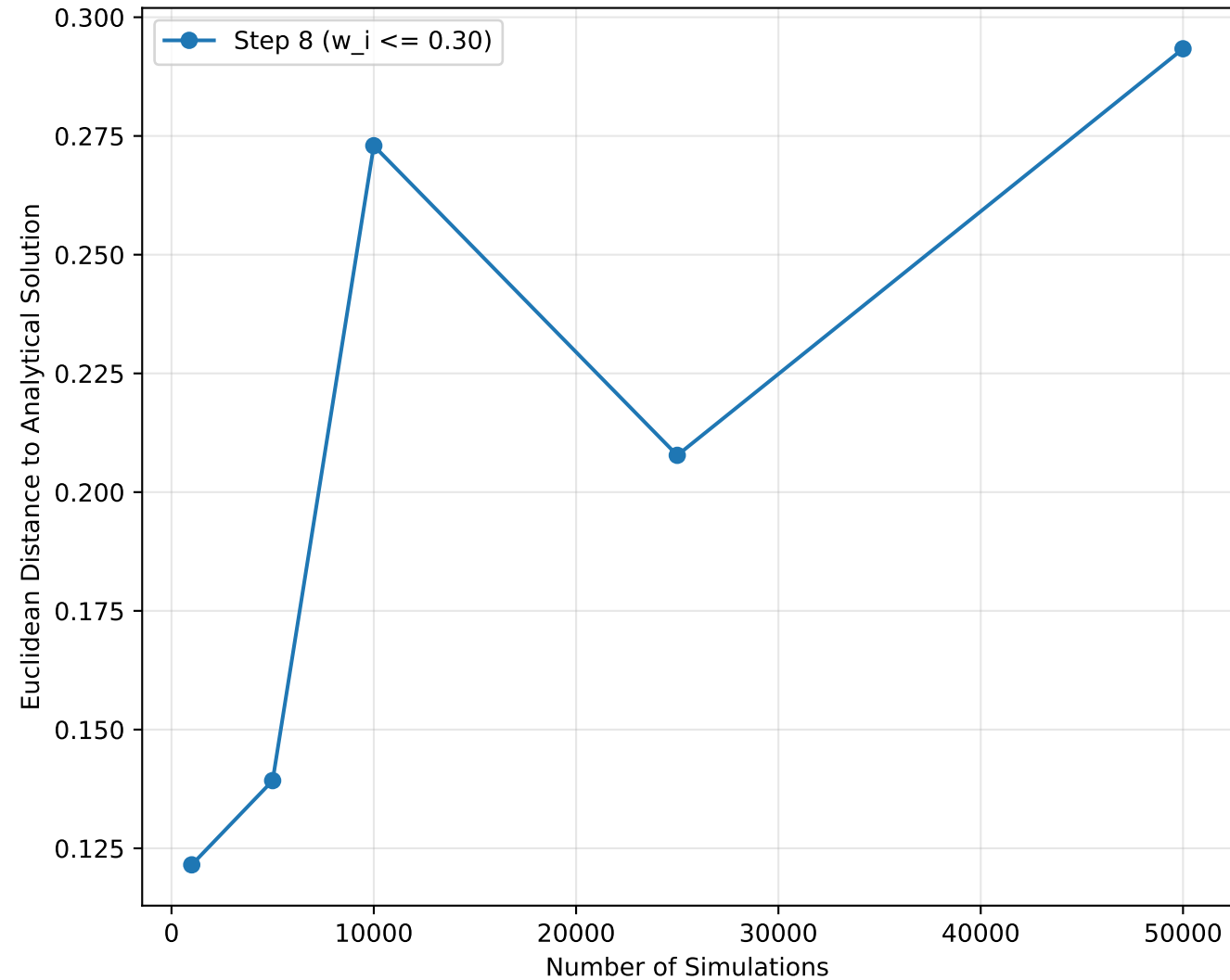
Step 8: Weight Convergence
