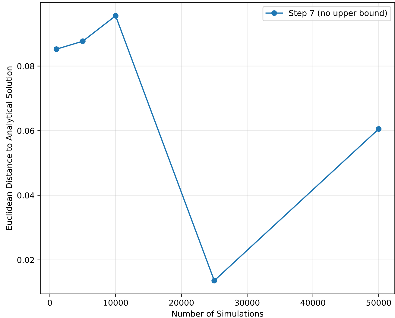
Step 7: Weight Convergence
