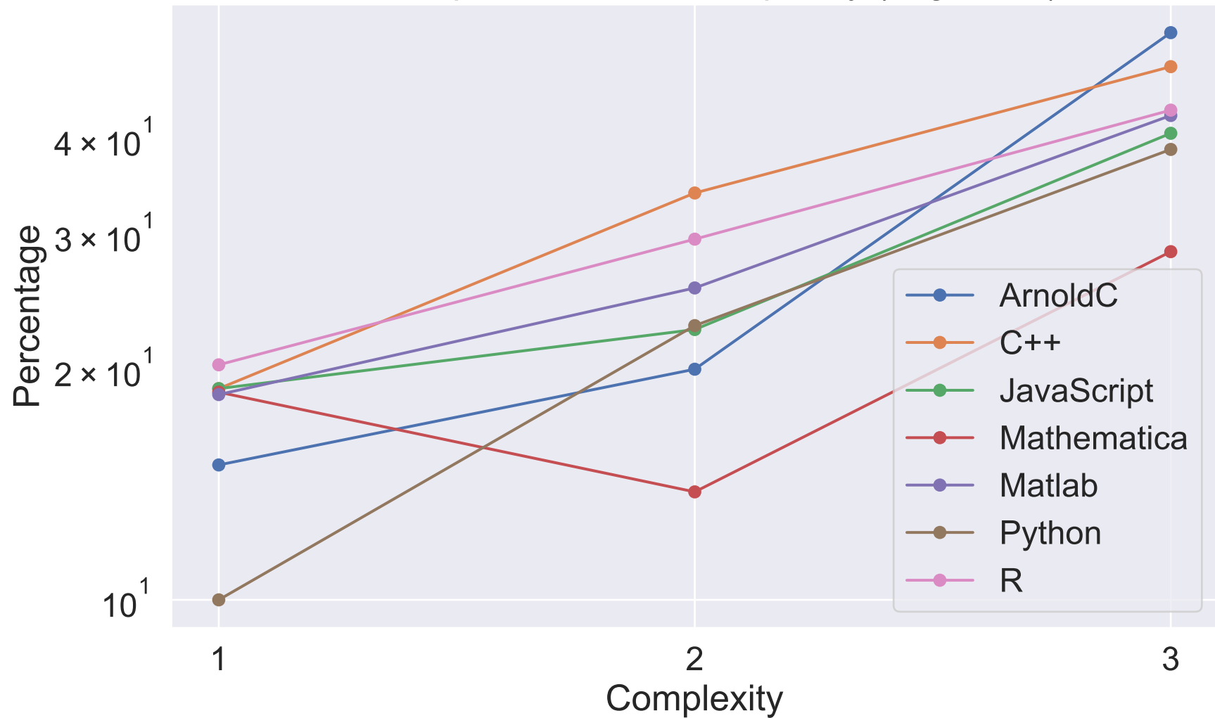
No compression % vs Complexity (Log Scale)
