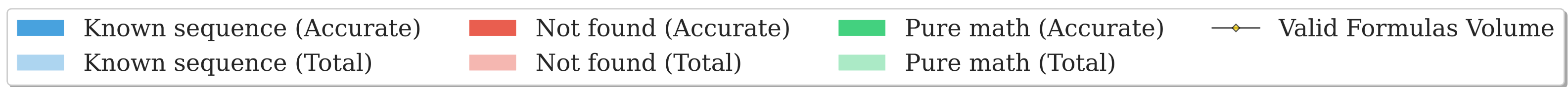
Complexity 1
