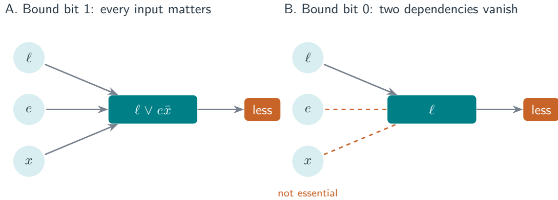
Figure 5: The comparator specialises itself. Both panels show the outgoing “less” of one comparison step, whose inputs are the incoming “less” \ell , the incoming “equal” e , and the value bit x . The cell is stated only as the meaning of a running comparison; the bound bit is a constant of the position, and nothing else is said. Against a bound bit of one the method finds all three inputs essential and names a two-clause form. Against a bound bit of zero it finds e and x inessential and returns \ell alone: below the bound one stays below, and no zero bound bit can create a new strict inequality. The orange dashed edges are the dependencies the method removed. They were not removed by an optimisation pass; the cofactor test simply did not find them.
