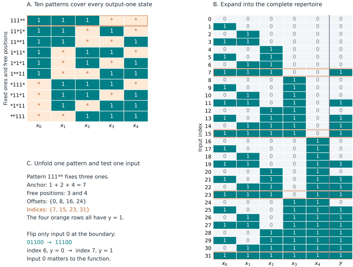
Figure 2: How do patterns recover the same output repertoire? Panel A shows the ten schemata, in Holland's sense [4], for the network in Figure 1. Teal entries are fixed ones; orange stars are don't-care positions, which may be zero or one. Panel B shows all 32 input states and the actual circuit output y = g_6 , ordered by input index. Orange outlines identify the four fillings of 111** . Panel C unfolds that pattern and shows a single-bit change that changes the output. The figure is generated from evaluated circuit states; the expanded schema union is checked against every output.
