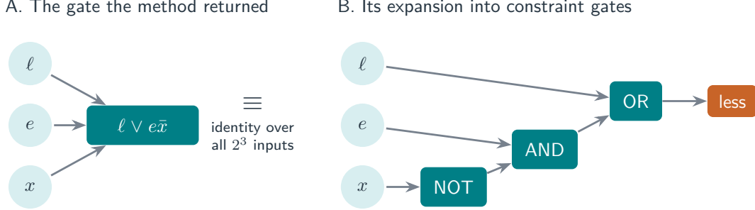
Figure 6: How does a recovered gate reach the constraint layer? Panel A is what deconvolution returned for one comparison step: a single gate of arity three, named as a two-clause form. The constraint layer does not carry that gate, so it must be folded into gates the layer does carry, shown in Panel B. The fold is not assumed correct. The expanded network is evaluated back into a decision-diagram root, the named gate is built independently by the engine’s own gate builder, and the two roots are compared: equal roots settle agreement on all eight inputs at once. A wrong fold cannot reach a constraint system, because the two roots would differ and the check would fail.
