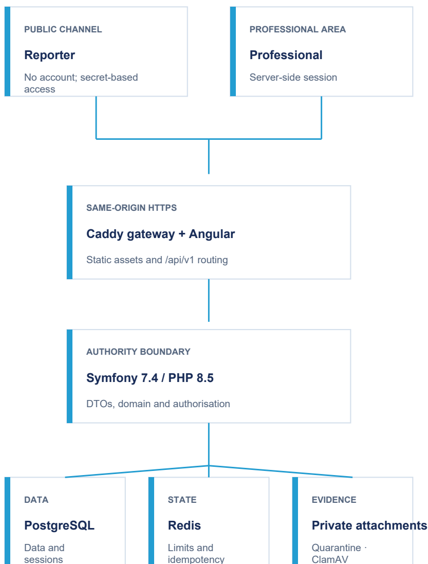
Figure 3. Logical architecture and authority boundaries.
