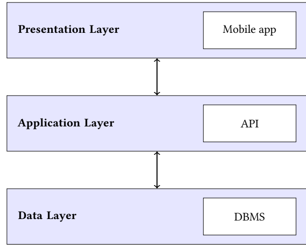
Figure 3: High-level three-layer architecture of GeoMedia, illustrating the separation of concerns between the Presentation Layer (mobile app interface), the Application Layer (backend API and logic), and the Data Layer (DBMS for data storage and retrieval).
