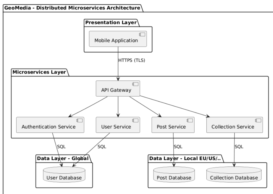
Figure 4.2: Microservices Software Architecture UML.
