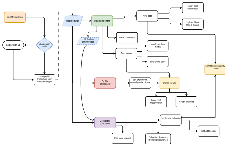
Figure 5.3: Application flowchart
