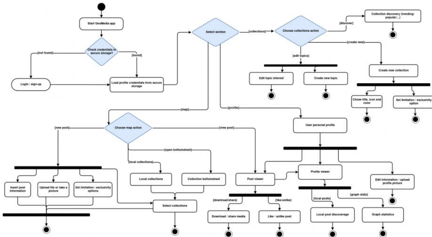
Figure 5.4: Activity diagram of GeoMedia app.
