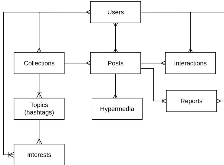
Figure 7.1: GeoMedia Entity-Relationship diagram
