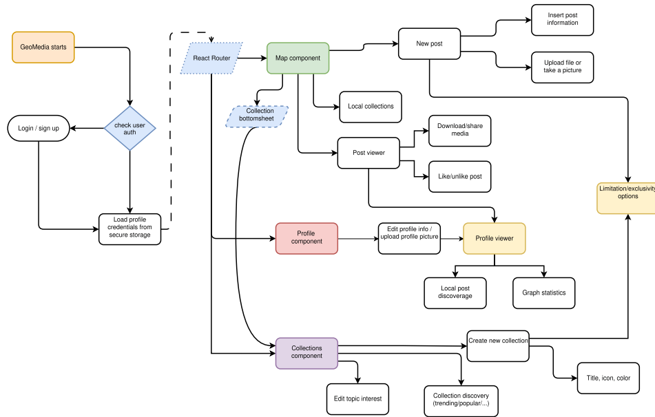
Figure 5.3: Application flowchart
