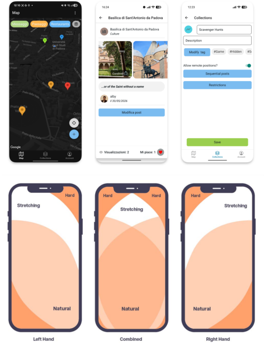
Figure 5.4: GeoMedia thumb-rule comparison
