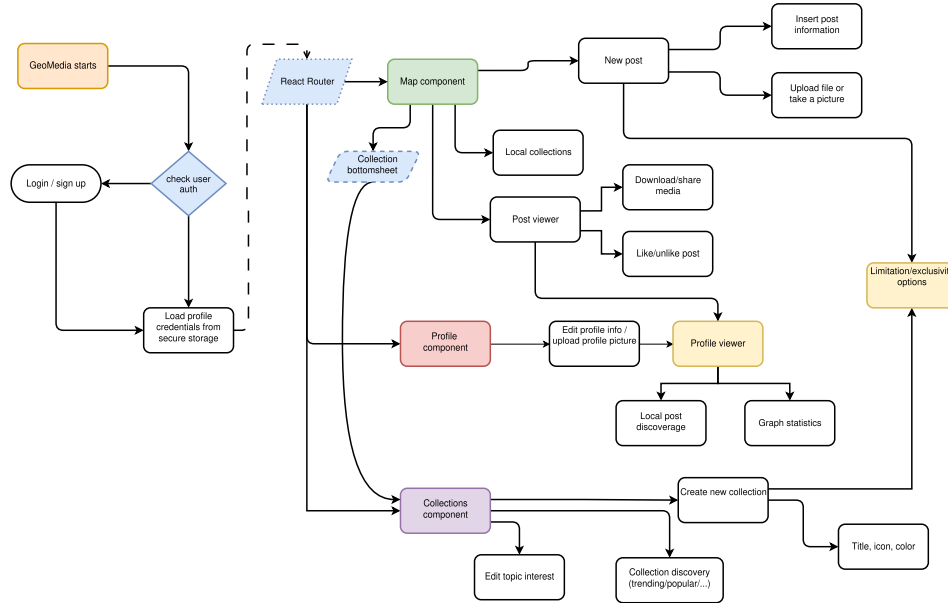
Figure 5.4: Application flowchart
