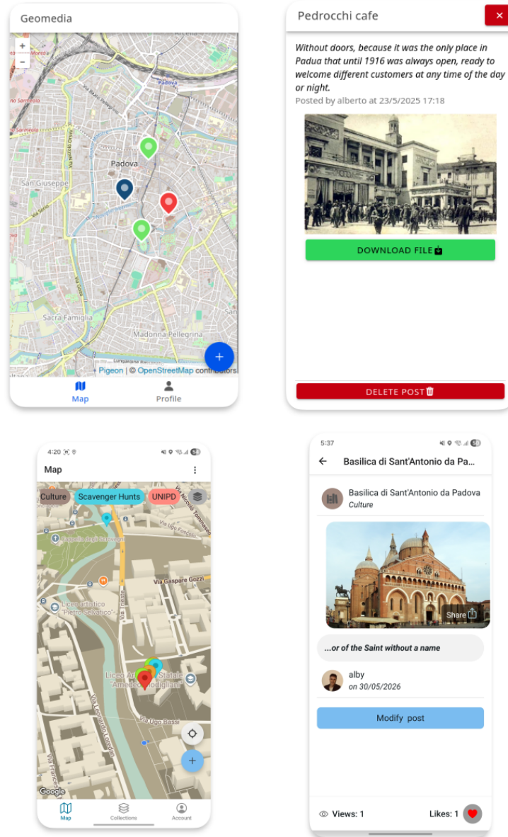
Figure 5.1: GeoMedia UI comparison between the Ionic Framework version (above) and the React Native version (below).
