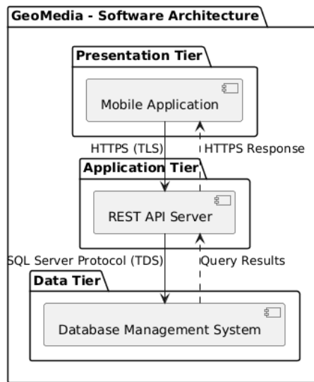
Figure 4.1: Three-tier Software Architecture UML.
