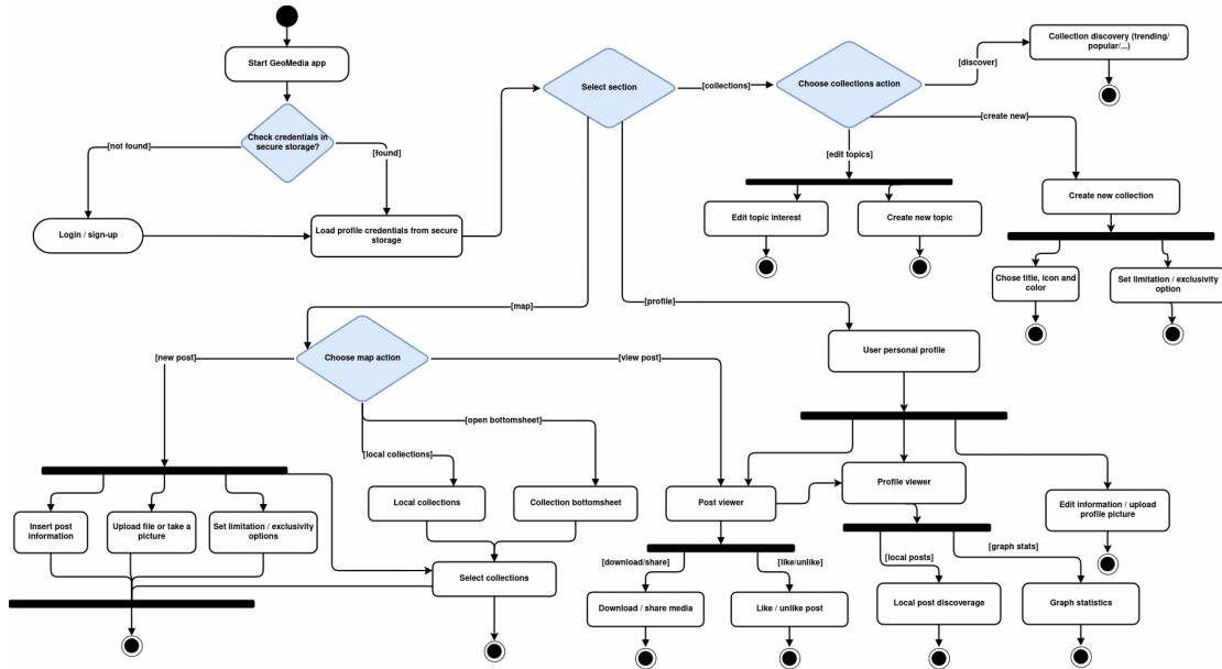
Figure 5.4: Activity diagram of GeoMedia app.
