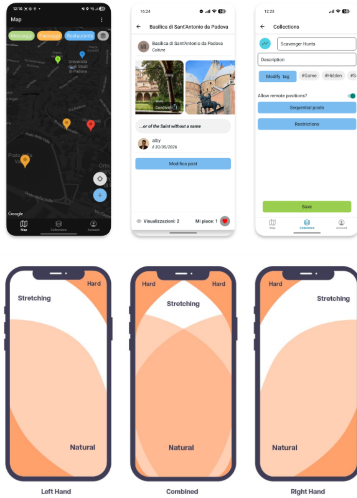
Figure 5.5: GeoMedia thumb-rule comparison [81]
