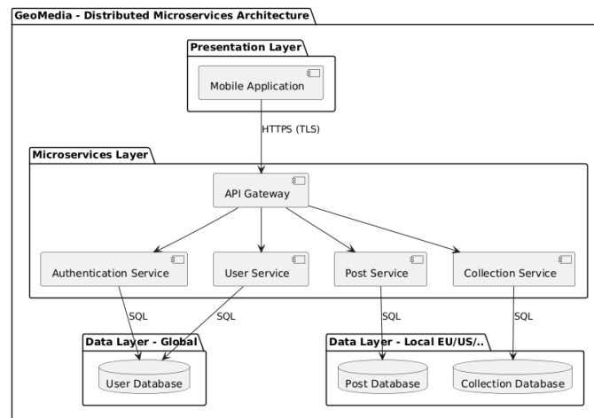
Figure 4.2: Microservices Software Architecture UML.
