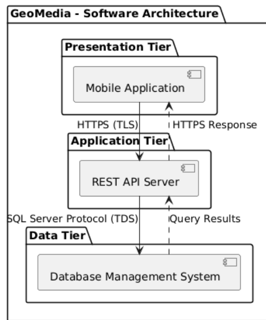
Figure 4.1: Three-tier Software Architecture UML.
