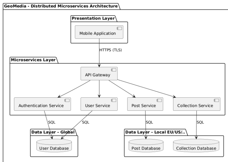
Figure 4.2: Microservices Software Architecture UML.
