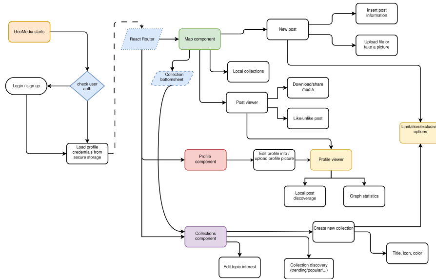
Figure 5.3: Application flowchart
