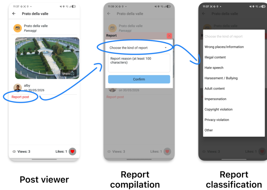
Figure 6.2: Post reporting.
