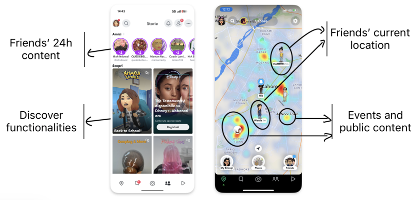
Figure 2.2: Snapchat functionalities
