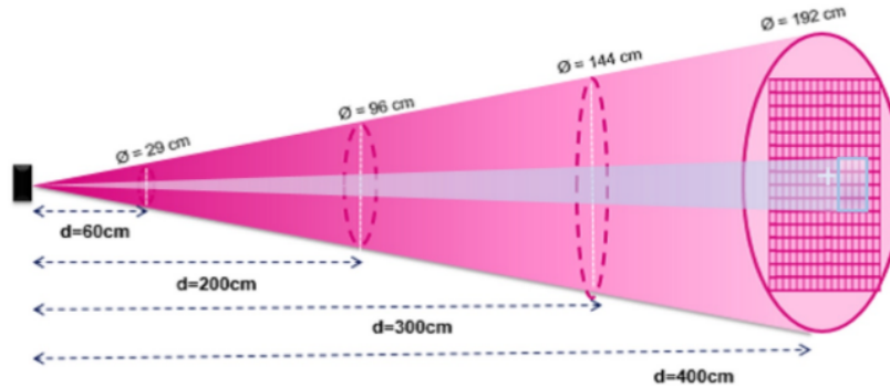
Figura 2.21: Field of View del VL53L1X
