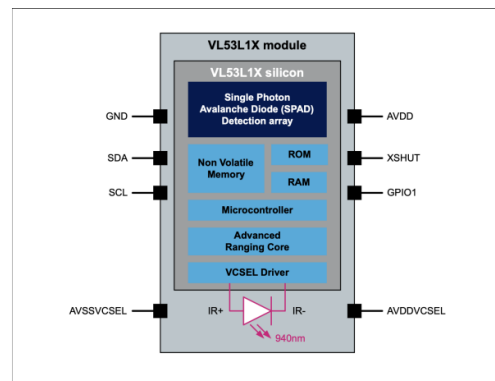
Figura 2.19: Pin Configuration (sinistra) e System Block Diagram (destra) del VL53L1X
