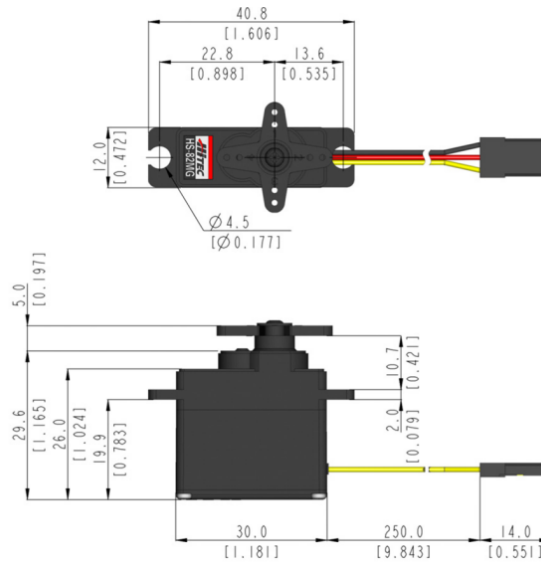
Figura 2.14: HS-82MG Hitec. Misure
