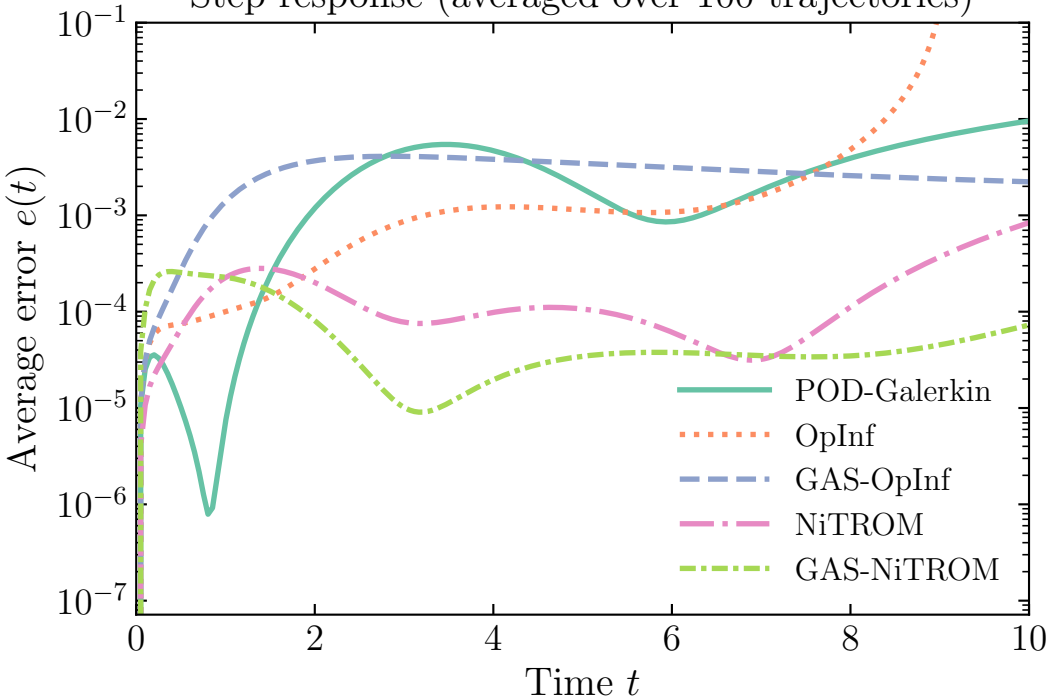
Step response (averaged over 100 trajectories)
