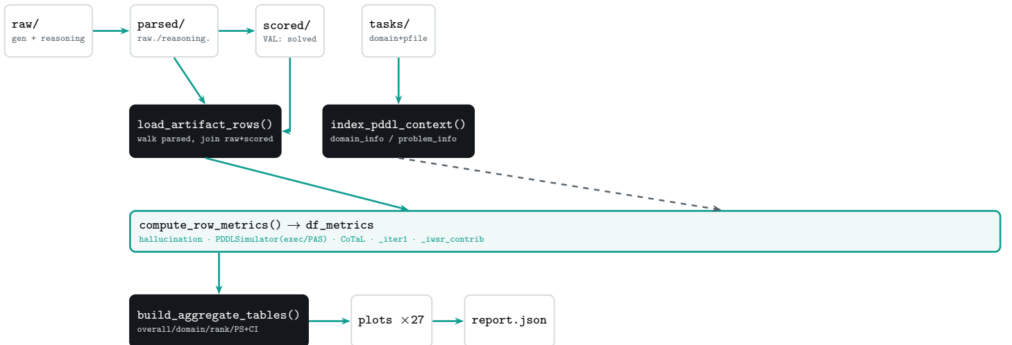
Figure 1: The analysis pipeline. One DataFrame, df_metrics , is the single source of truth; PDDL ground truth (dashed) is injected to score plans.
