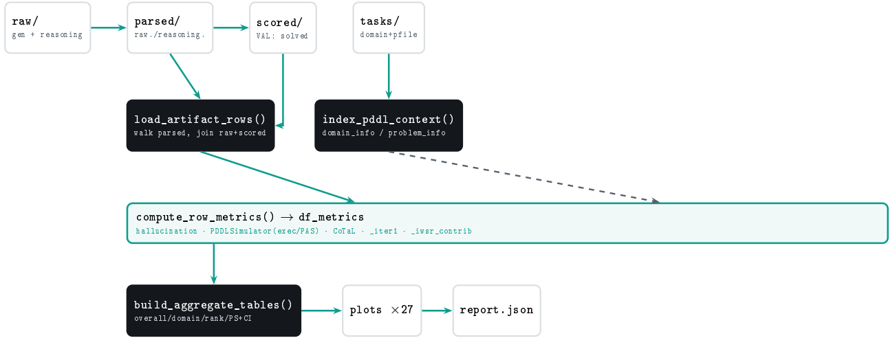
Figure 5: The analysis pipeline. One DataFrame, df_metrics , is the single source of truth; PDDL ground truth (dashed) is injected to score plans.
