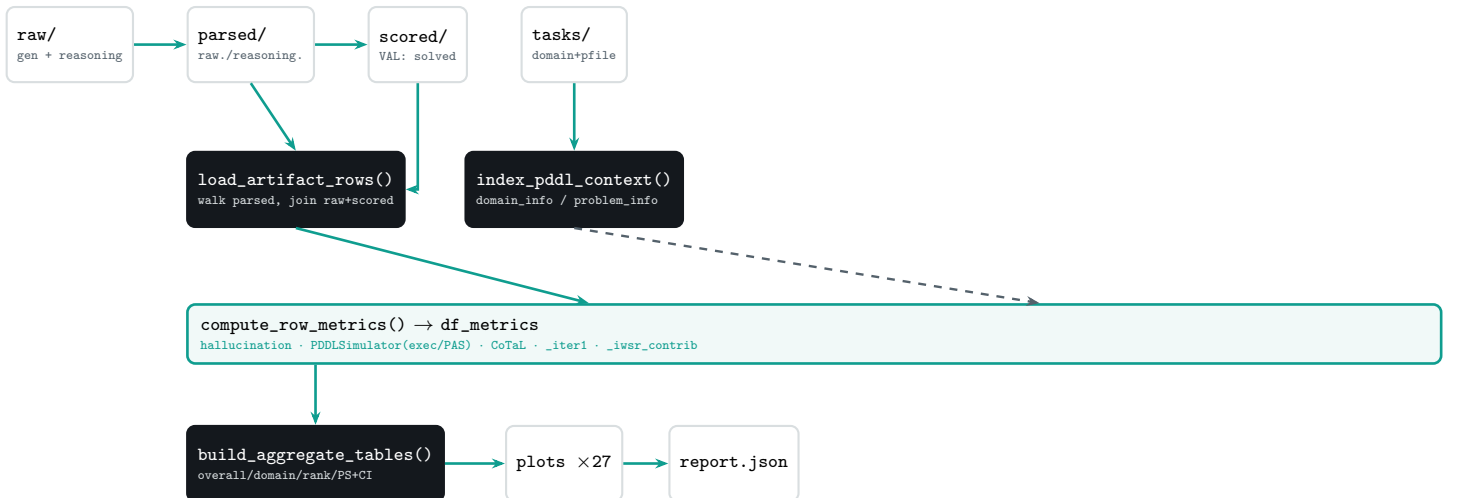
Figure 1: The analysis pipeline. One DataFrame, df_metrics , is the single source of truth; PDDL ground truth (dashed) is injected to score plans.
