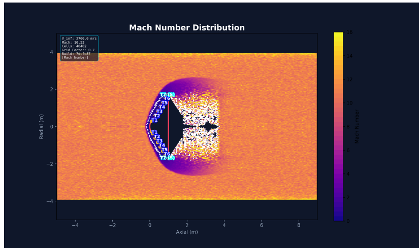
Figure 4.3: Mach number field around the HIAD showing bow shock structure and subsonic regions.
