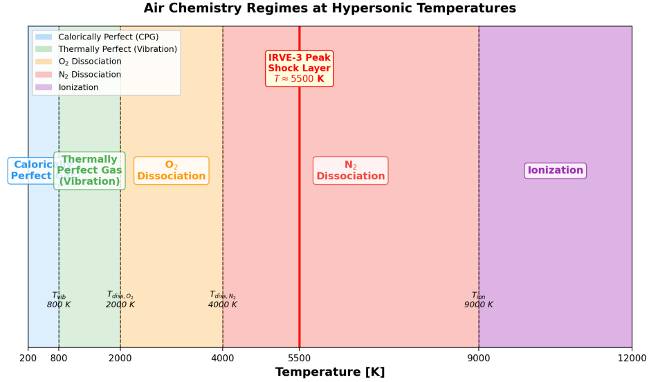
Figure 2.17: Air chemistry regimes as a function of temperature, showing vibrational excitation, molecular dissociation, and ionization thresholds (, ).
