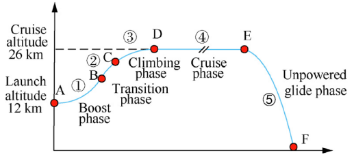
Fig. 2 Mission profile of AHV.
