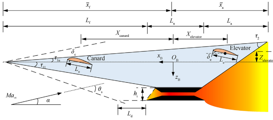
Fig. 1 Geometry configuration of AHV. 16,17
