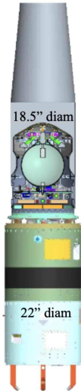
Figure 3.7: Launch configuration of the HIAD system, showing the stowed constraint.
