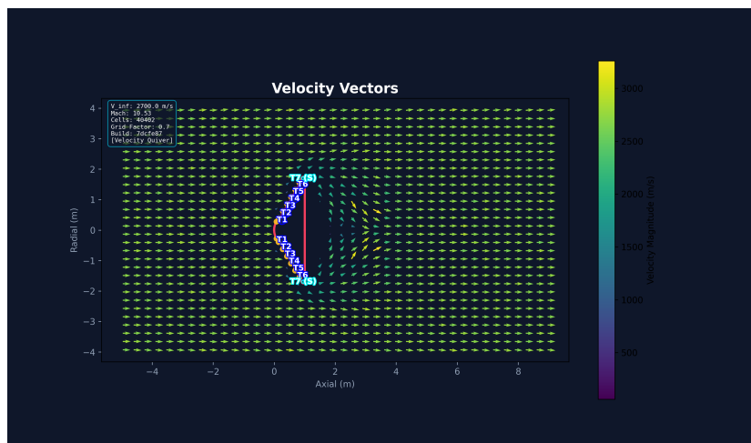
Figure 4.4: Velocity vector field showing recirculation zones in the toroidal valleys.
