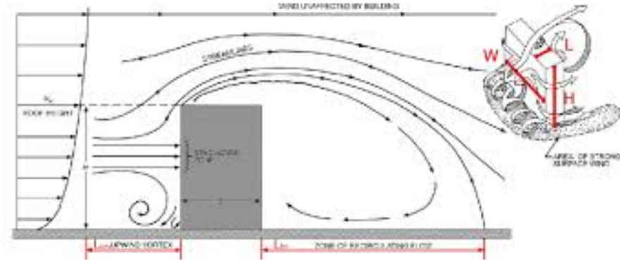
Figure 2.13: Figure for Recirculation Zones and Stagnation Valleys Example on different scenarios.
