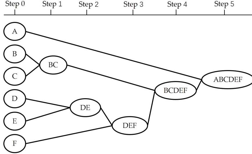
Figure 1: Agglomerative clustering
