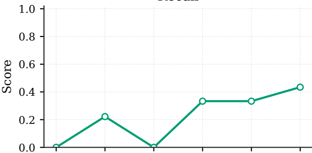
Recall
