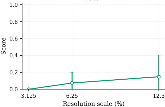
Recall
