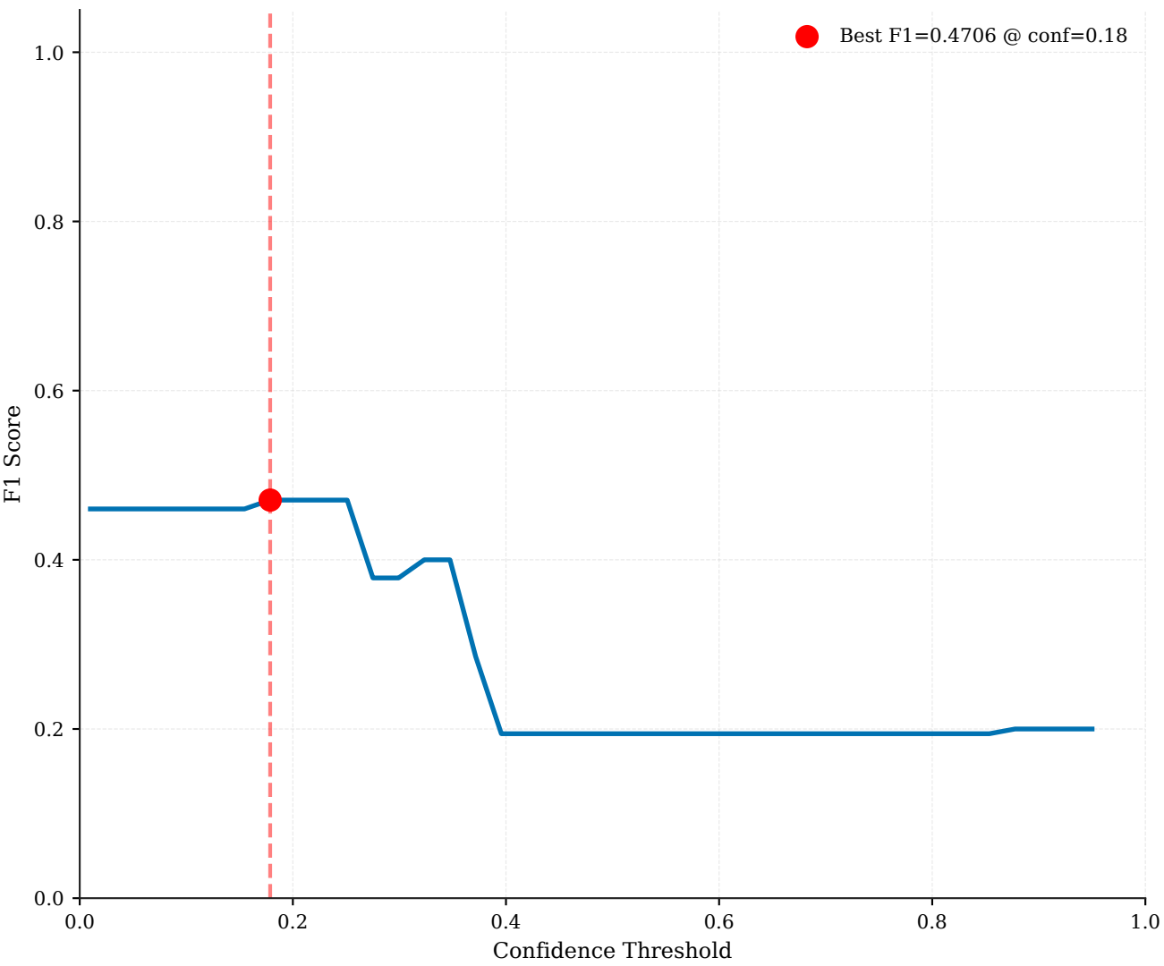
F1-Confidence Curve
